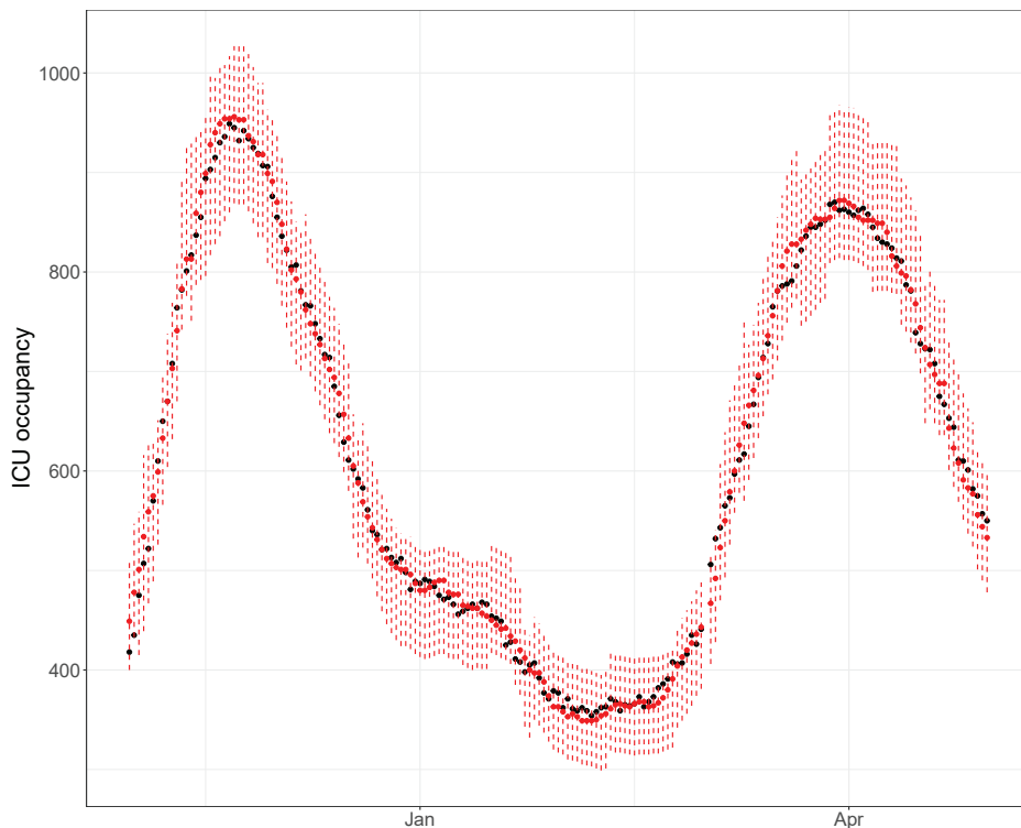
Figure 2: Observed (black dots) and predicted (red dots) with 95% confidence intervals (red dashed lines) for ICU occupancy in Lombardy during the second and the third wave of Italy's Covid-19 epidemic, 1 November 2020 to 30 April 2021.
